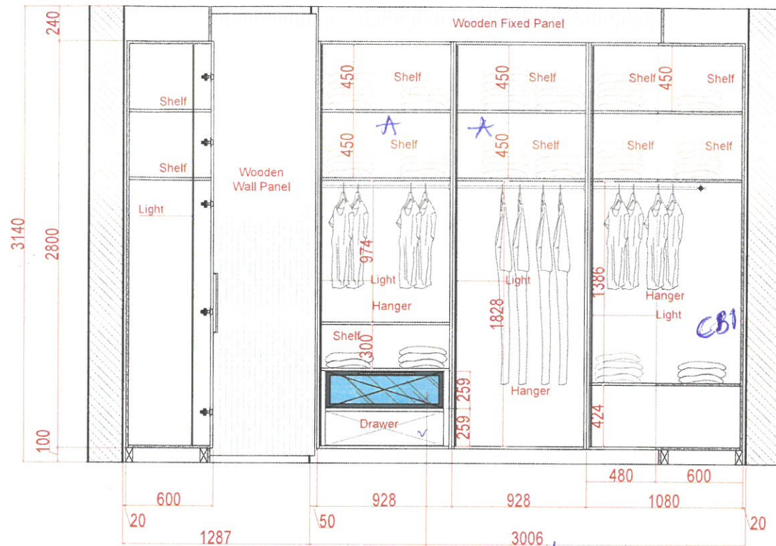
Elevation- A Details Drawer Face with Aluminum Frame with Glass without Top
