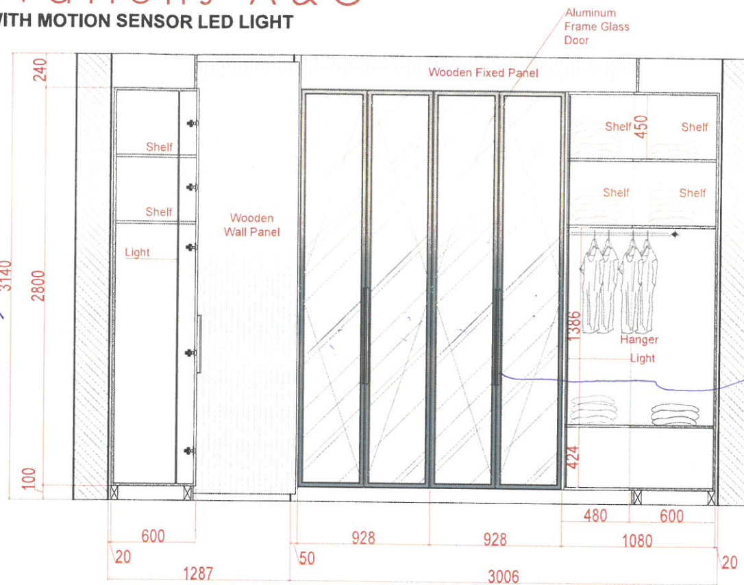
Elevation- A Details with Door Aluminum Frame Glass Door
