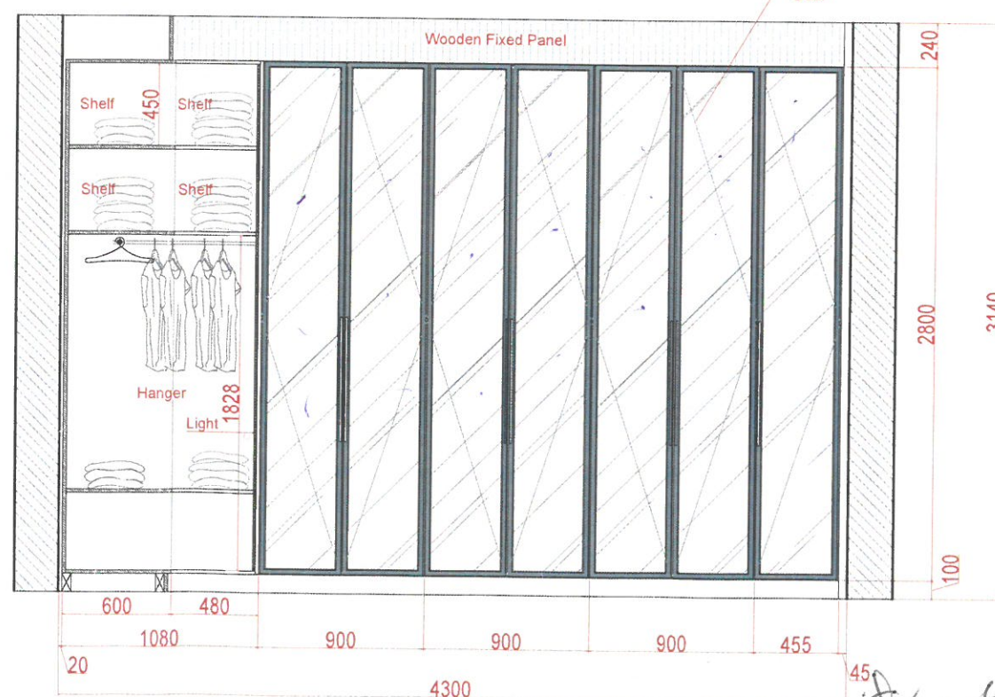
Elevation- C Details with Door
