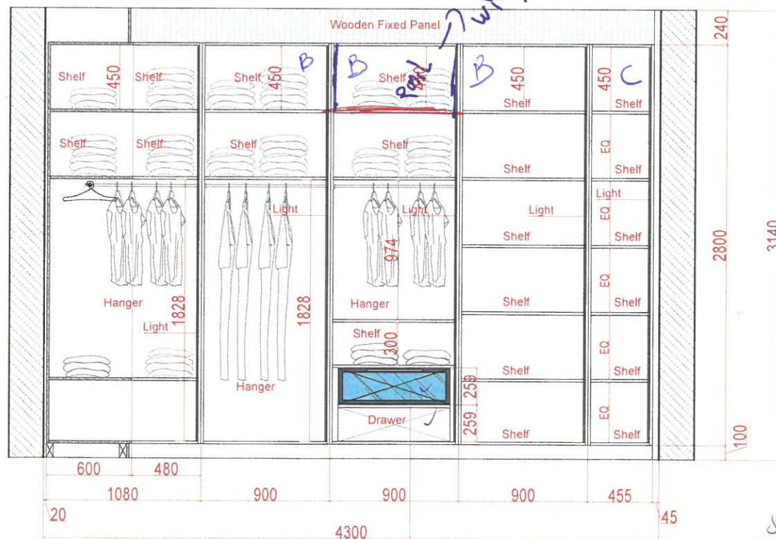
Elevation- C Details
